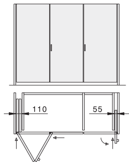
与Hawa concepta III 25/35 pull相结合的三门系统, 带底部型材
